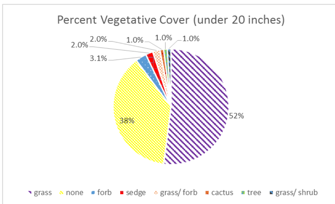
Figure 4. Percent Vegetative Cover for plot on 15-08.
