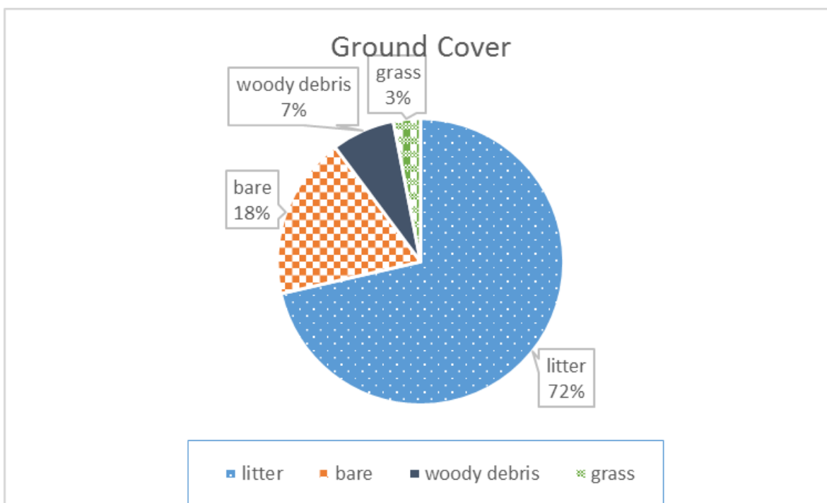
Figure 6. Percent ground cover for plot on 15-08.
