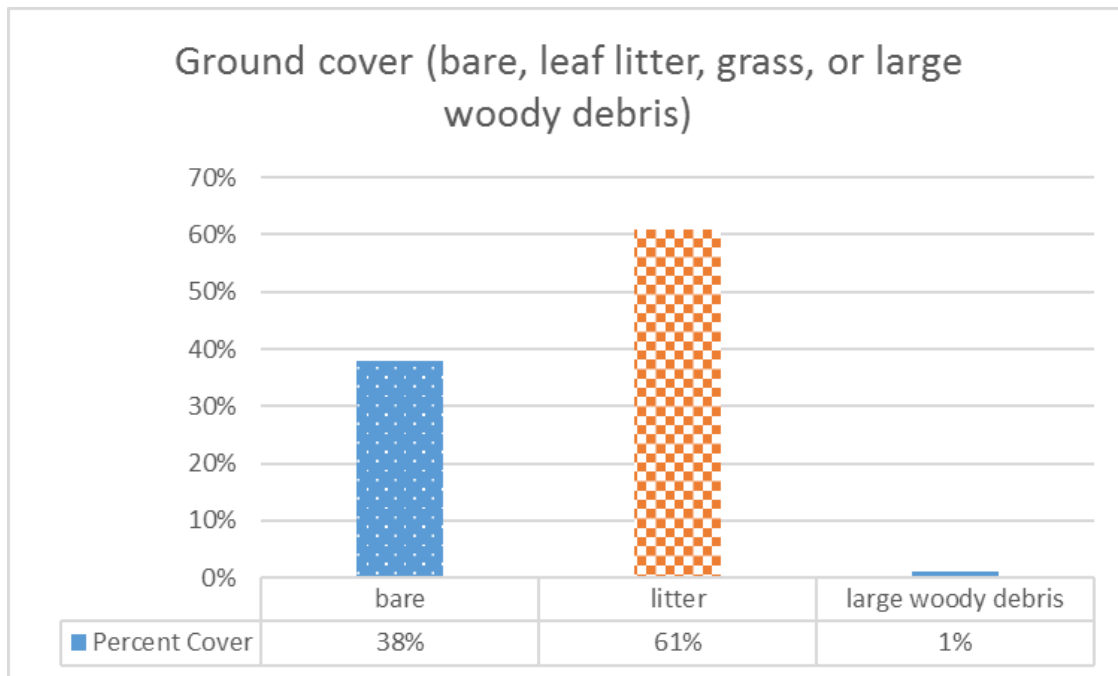
Figure 8. Percent ground cover for plot on 16-12.
