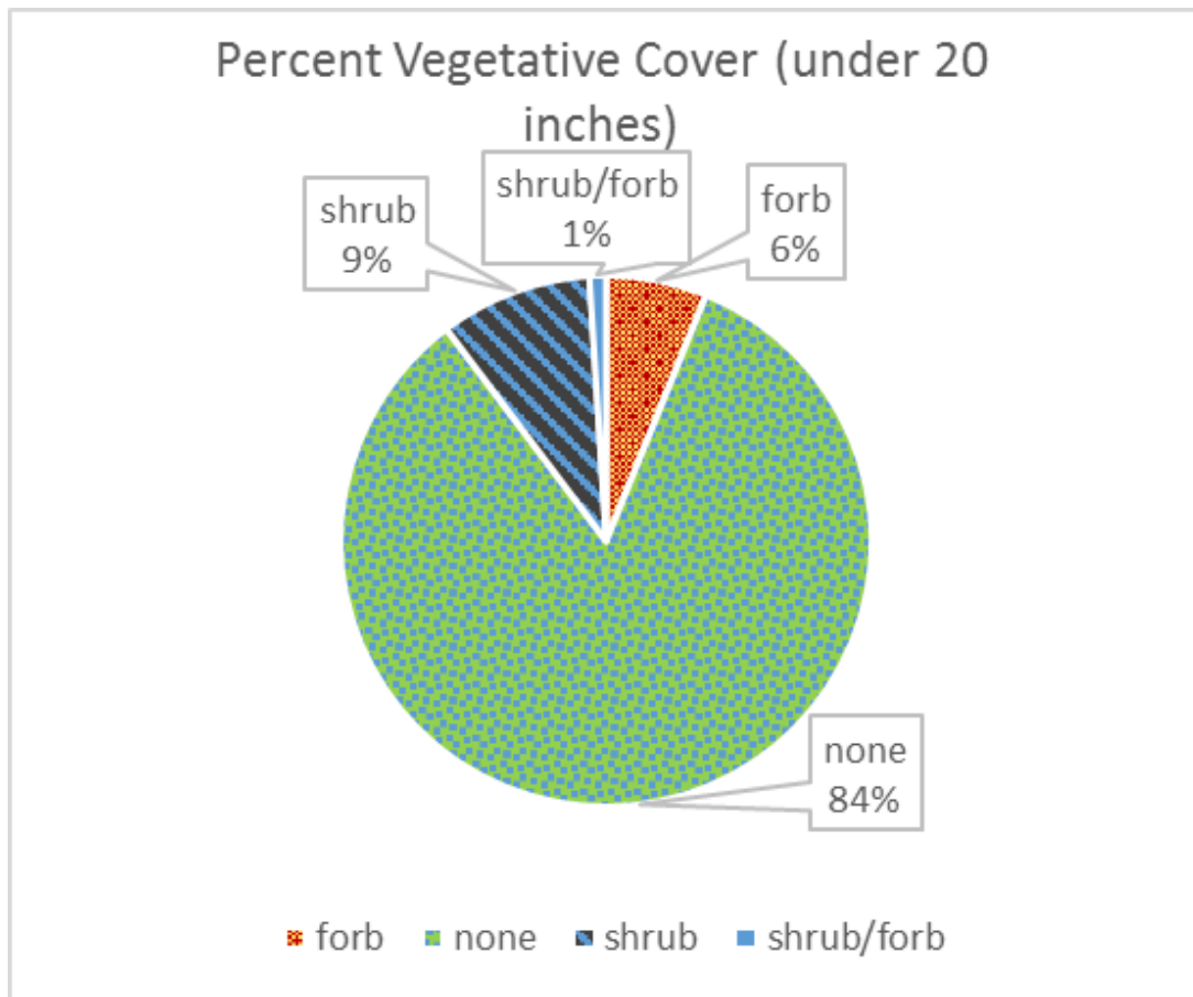
Figure 5. Percent Vegetative Cover for plot on 16-12.
