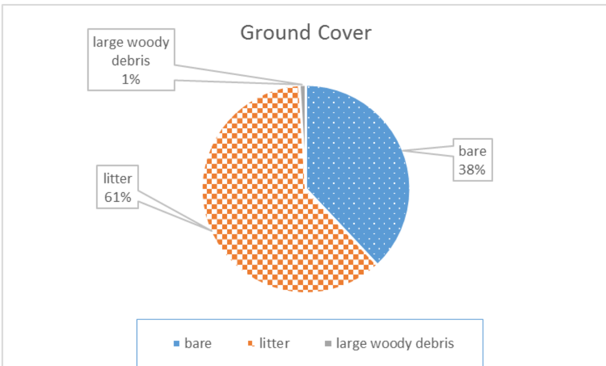
Figure 7. Percent ground cover for plot on 16-12.
