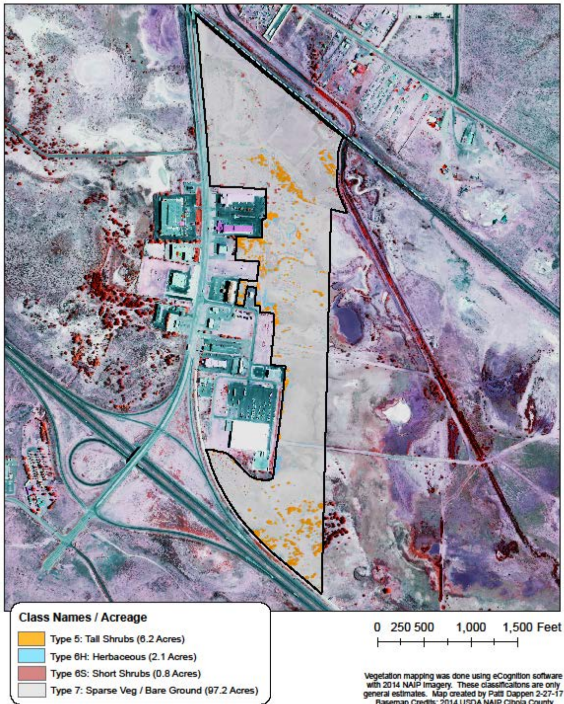
Figure 4. NAIP vegetation classification for 16-12.
