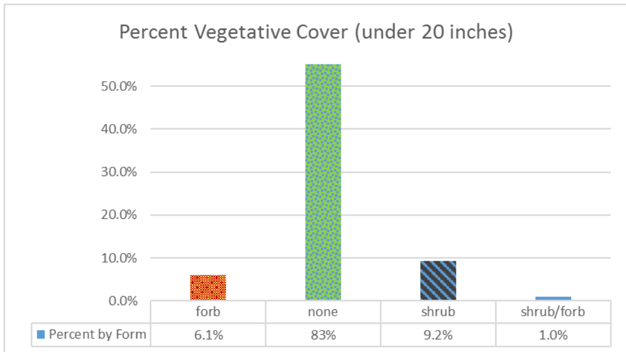
Figure 6. Percent Vegetative Cover for plot on 16-12.
