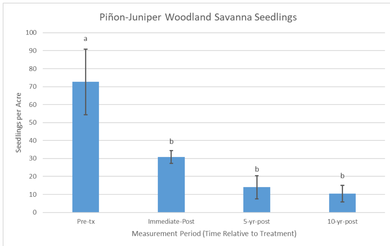
Figure III.19 Analysis of Variance (ANOVA) Results for Piñon-Juniper Woodland Savana Live Seedlings per Acre. Data displayed are means ( \pm standard error of the mean) for each measurement period. Means marked with the same letter do not differ significantly ( \alpha = 0.05 ) according to Tukey's Honest Significant Difference multiple pairwise comparison.
