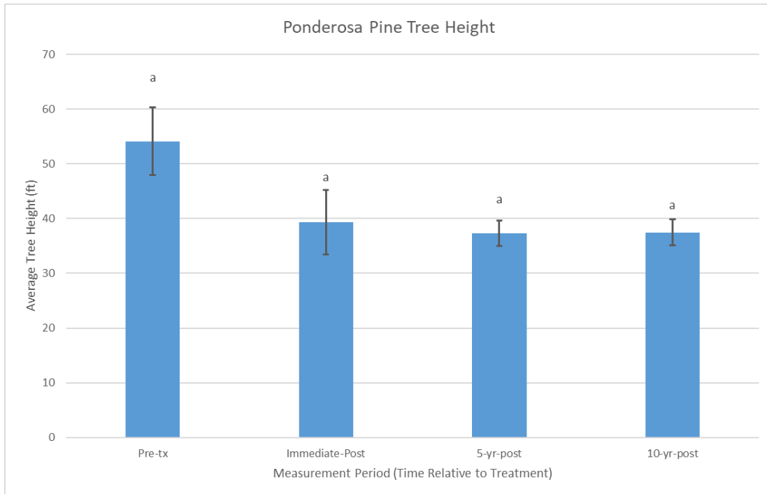
Figure III.9 Analysis of Variance (ANOVA) Results for Ponderosa Pine Tree Height.
