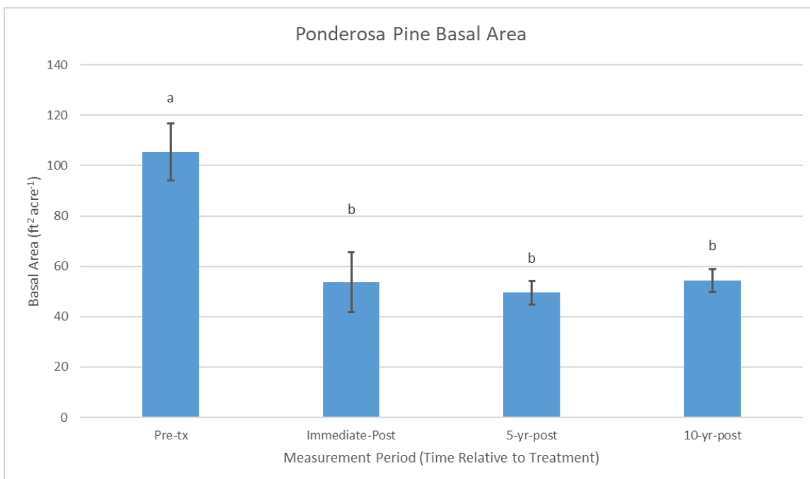
Figure III.8 Analysis of Variance (ANOVA) Results for Ponderosa Pine Basal Area.
