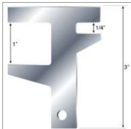
Figure 7. Go-no-go Gauge
