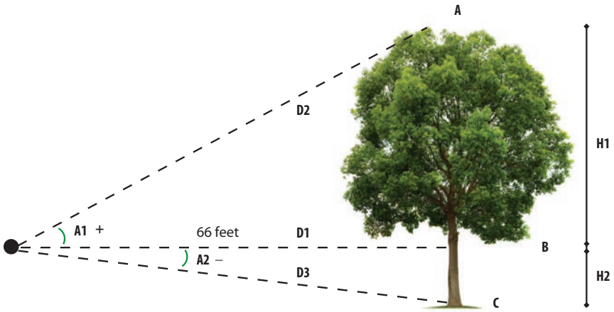
FIGURE 11. CLINOMETER USE (ADAPTED FROM USFS, 2010B)
