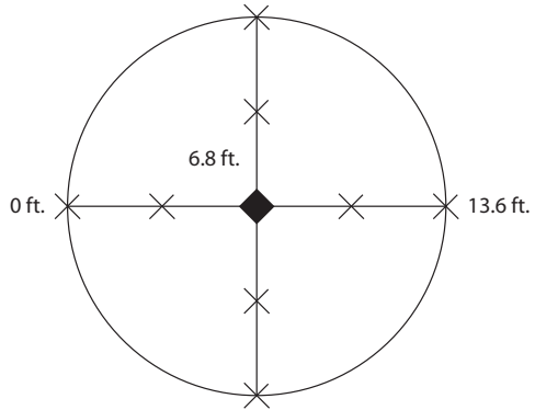
FIGURE 6. SMALL PLOT LAYOUT (1/300 ACRE)
