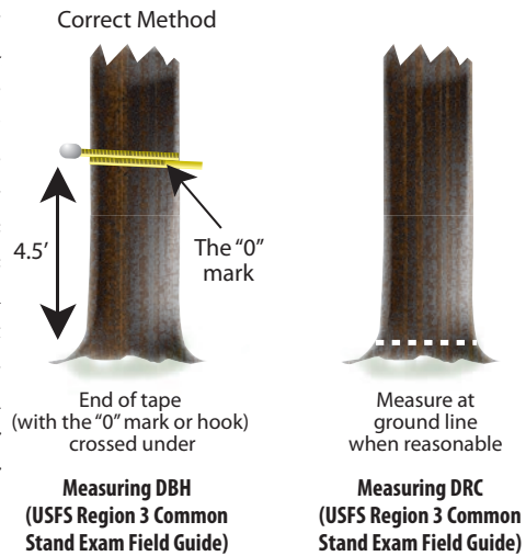
FIGURE 10. DBH AND DRC MEASUREMENT
