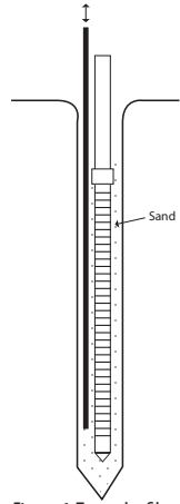
Figure 6: Tamp the filter pack.
