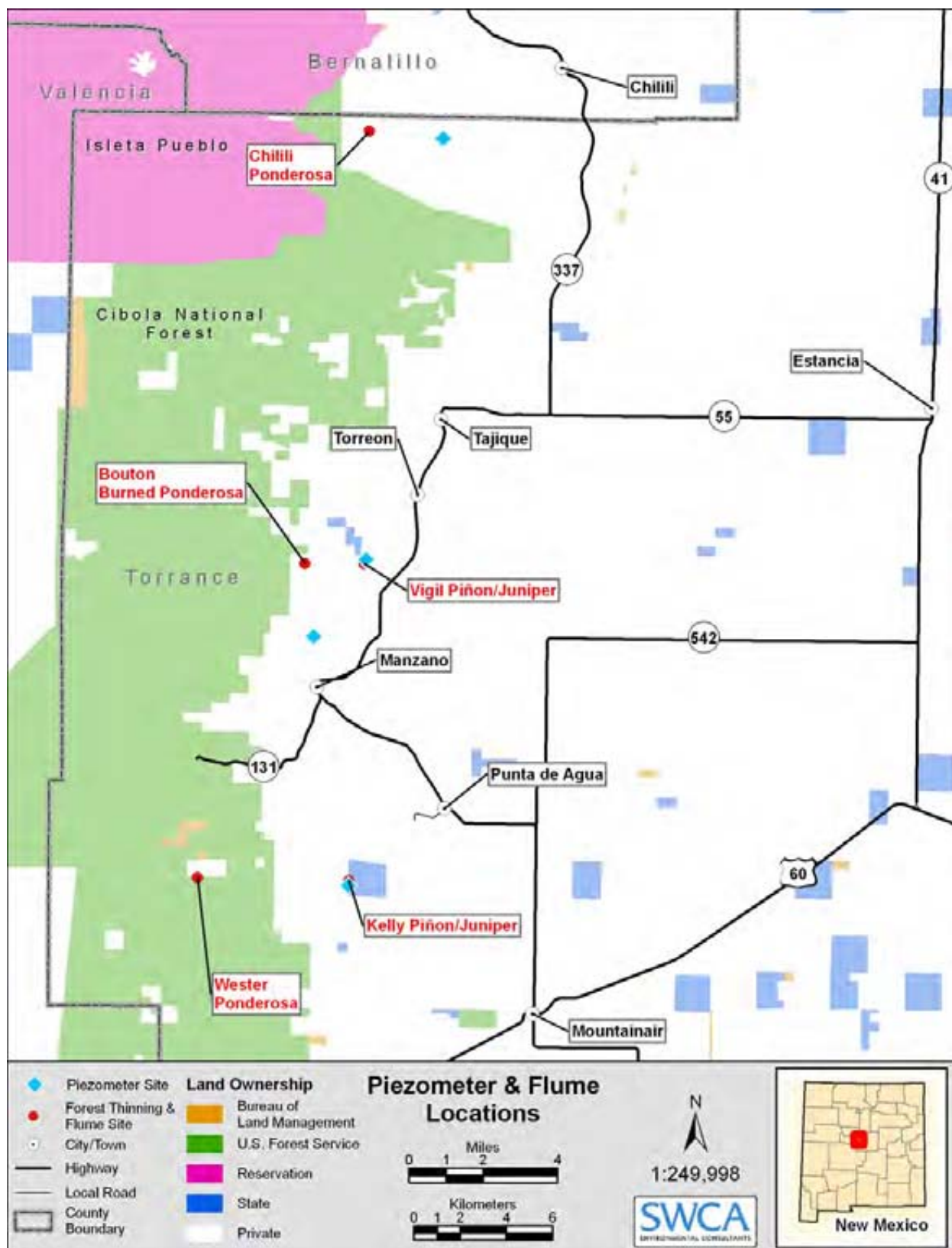
Figure 22. Flume locations.
